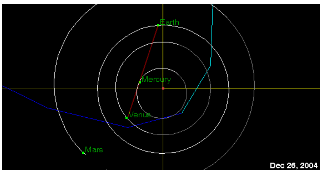
Figure 4. Astronomical alignment (red) Earth-Mercury-Venus on day of M9.1 Indonesia quake of 26-Dec-2004, Table 2.
