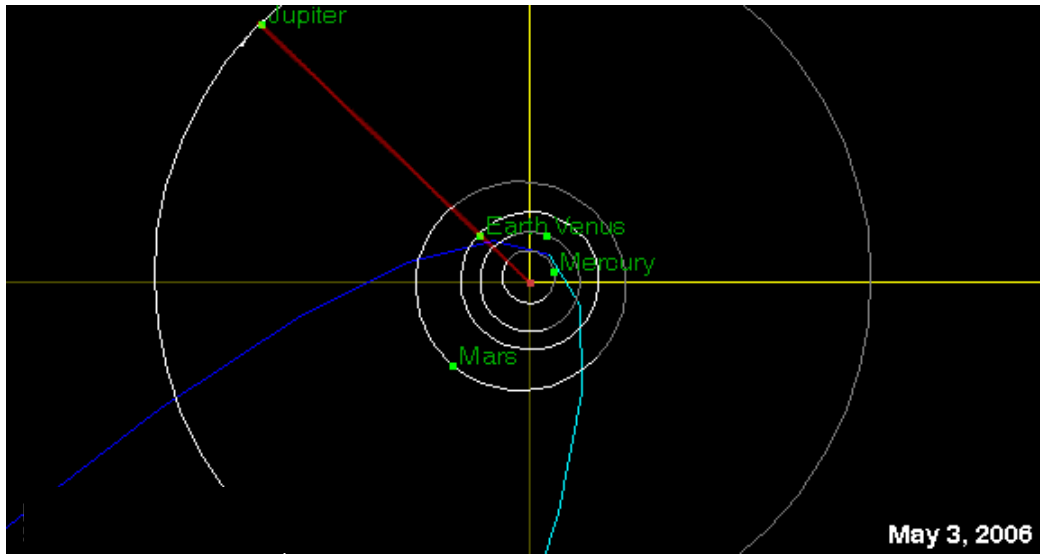
Figure 5. Astronomical alignment (red) Jupiter-Earth-Sun on the day of M8 Tonga earthquake of 03-May-2006, Table 2.
