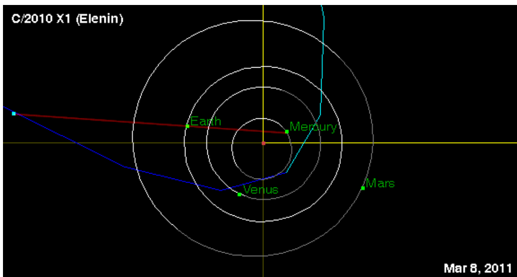
Figure 7. Astronomical alignment (red) Elenin-Earth-Mercury, -3 day of M9 Japan earthquake of 11-Mar-2011, Table 2.
