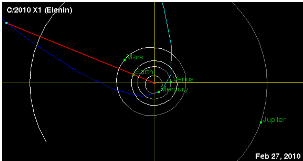
Figure 6. Astronomical alignment (red) Elenin-Earth-Sun on the day of M8.8 Chile earthquake of 27-Feb-2010, Table 2.
